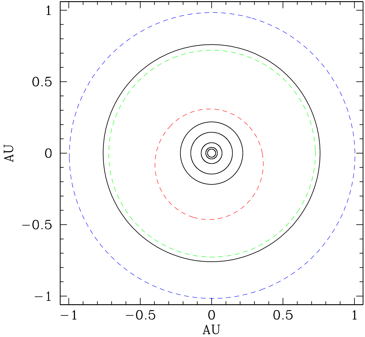
Fig. 6.— Top view of the GJ 581 system. For reference, the orbits of Earth, Venus, and Mercury are overlaid as dashed blue, green, and red lines respectively.
