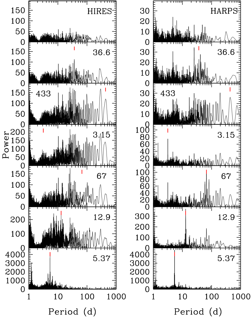
Fig. 4.— The effect of sequentially adding signal in reverse order at each Keplerian period back into the residuals of each data set for GJ 581. Panels on the left show the results for the HIRES data set, while those on the right show the results for the HARPS data set. The top panels show the periodograms of the residuals from the 6-planet fit. The annotations and red vertical tick marks in each panel indicate the period of the last injected signal prior to computing each periodogram.
