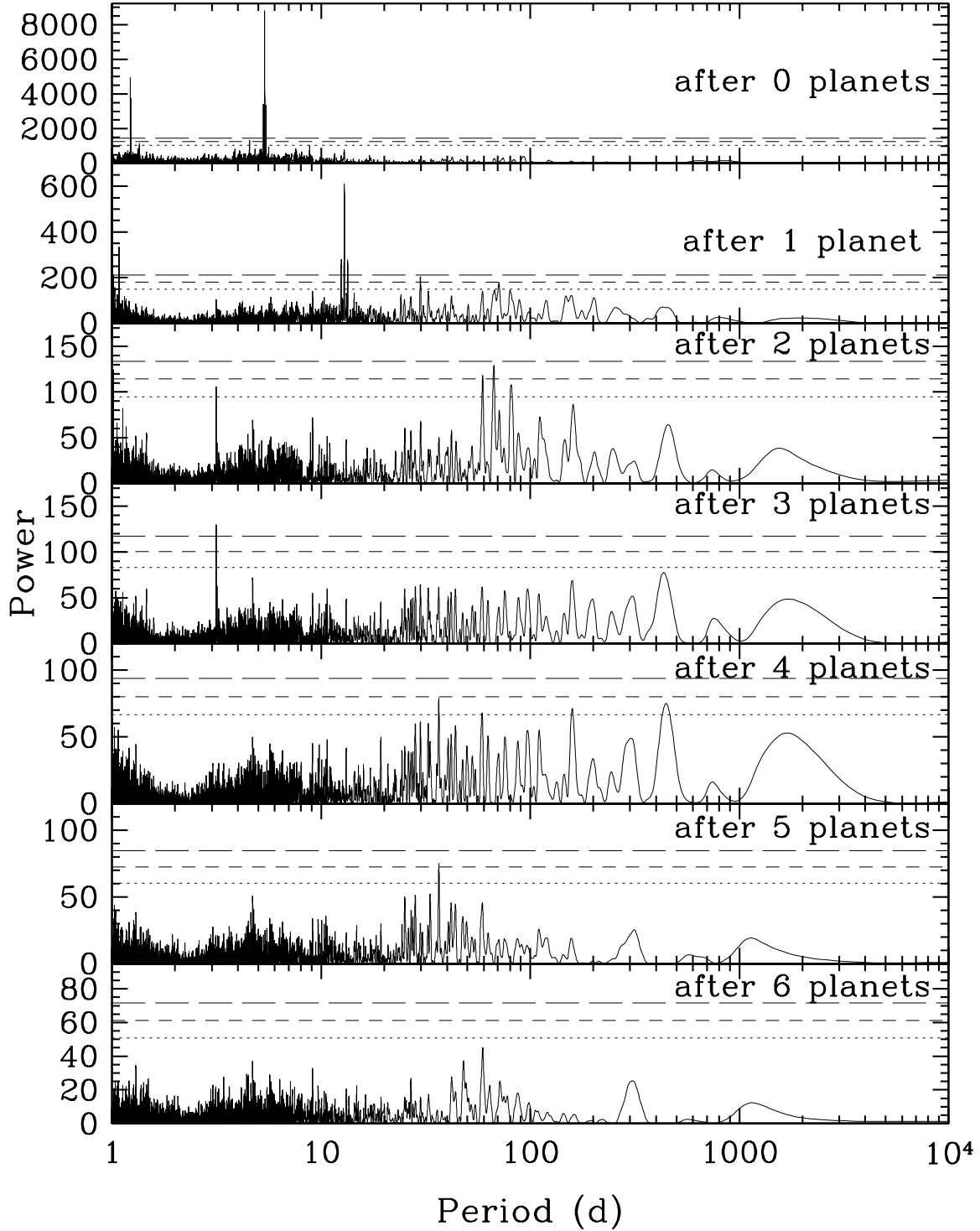
Fig. 3.— From top to bottom, power spectra of the residuals to the 0-, 1-, 2-, 3-, 4-, 5-, and 6-planet solutions, respectively. The horizontal lines in each periodogram roughly indicate the 0.1%, 1.0%, and 10.0% False Alarm Probability (FAP) levels from top to bottom.
